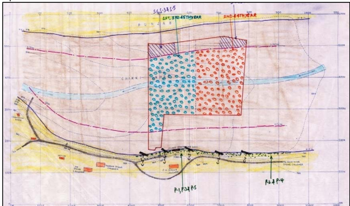
FIGURE-2.5: CONTOUR AND WORKING PLAN OF THE MINING LEASE AREA.
